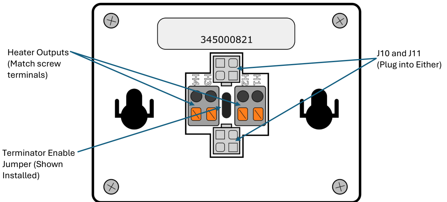
Figure 3 - Back of EasyTouch RV 345
